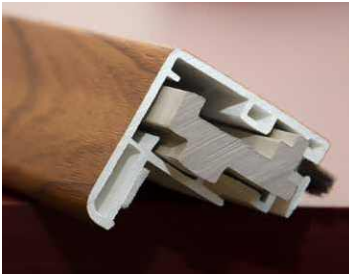
Additional High Density Composite Reinforcement Reinforcement inside the locking sash makes our windows structurally stronger than others available on the market.
